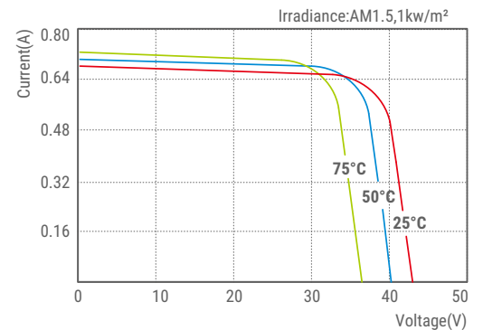
SLP020S-24U I-V Curves
